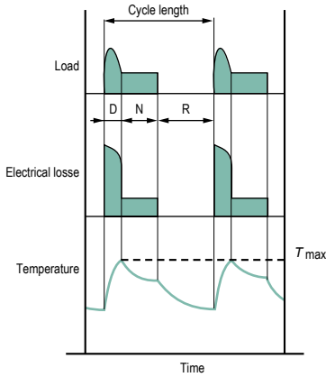
Fig. 4. - Intermittent periodic duty with starting, Type S4.
