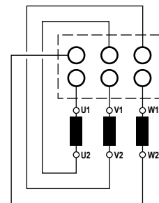
Internal wiring diagram
