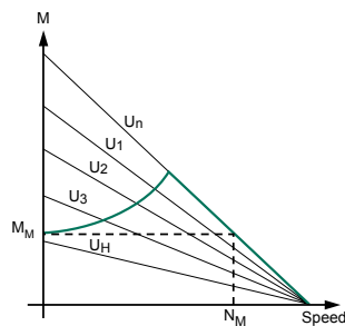
Characteristic curves of a high-torque motor
