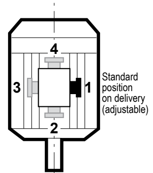
Positions of the cable gland in relation to the drive end
