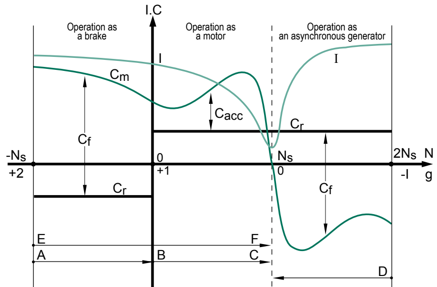
Curves I = f(N) , C_m = f(N) , C_f = f(N) , in the motor starting and braking zones.
