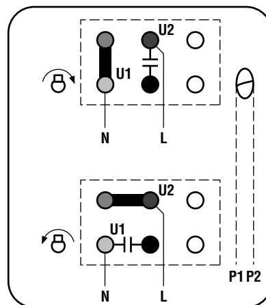
Single phase motor with permanent capacitor
