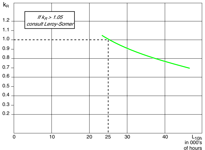
▼ Change in bearing life L_{10h} according to the radial load factor k_R for standard assemblies.
